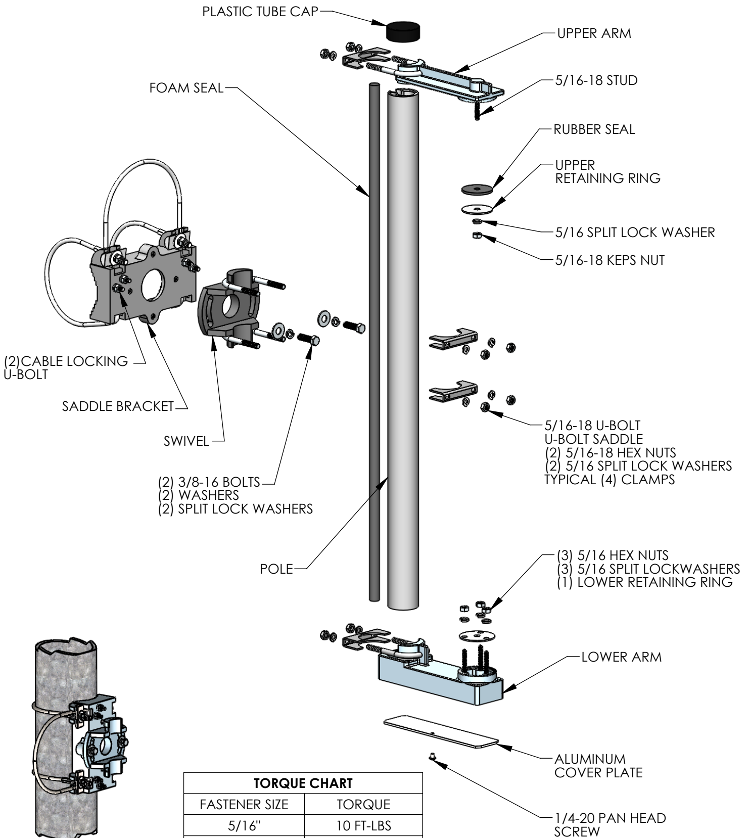
ALTERNATE MOUNTING
