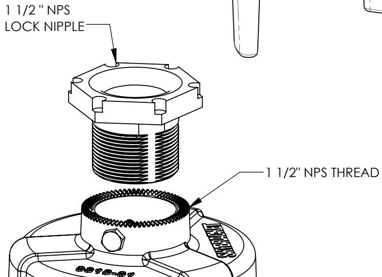
LOCK NIPPLE DETAIL
